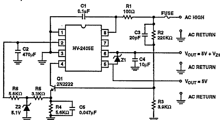
FIGURE 15. DUAL SUPPLY
