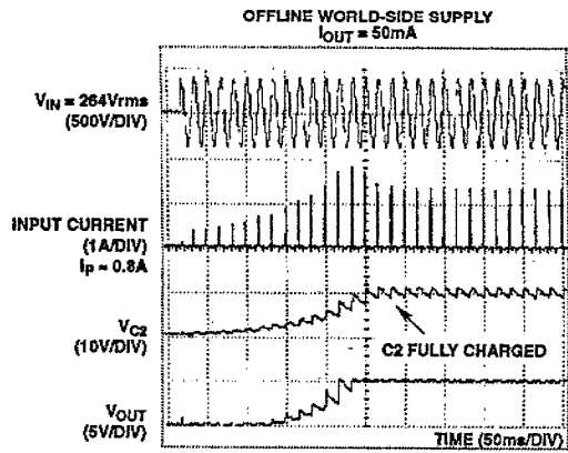
FIGURE 2. START UP OPERATION
