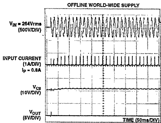
FIGURE 3. SHORT CIRCUIT OPERATION
