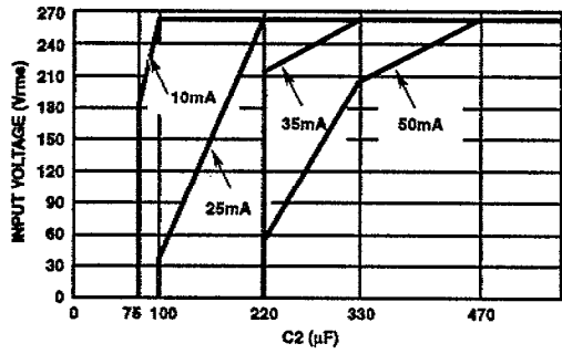
FIGURE 19. MINIMUM C2 VALUE vs INPUT VOLTAGE 50Hz
